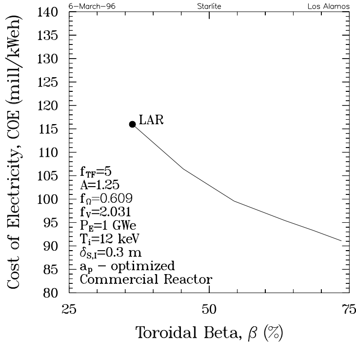
Figure 8.4-8. The cost of electricity for LAR parameters as a function of the plasma \beta . Note that this variation is not based on self-consistent plasma equilibria. Rather the achievable \beta of the base equilibrium (36%) is arbitrarily increased.
