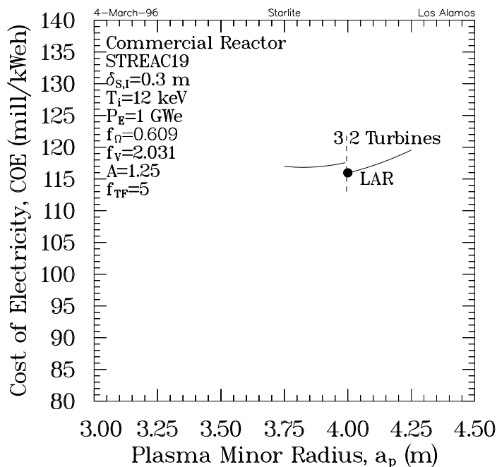
Figure 8.4-2. Cost of electricity as a function of plasma minor radius calculated internally to the ASC for the given LAR parameters.
