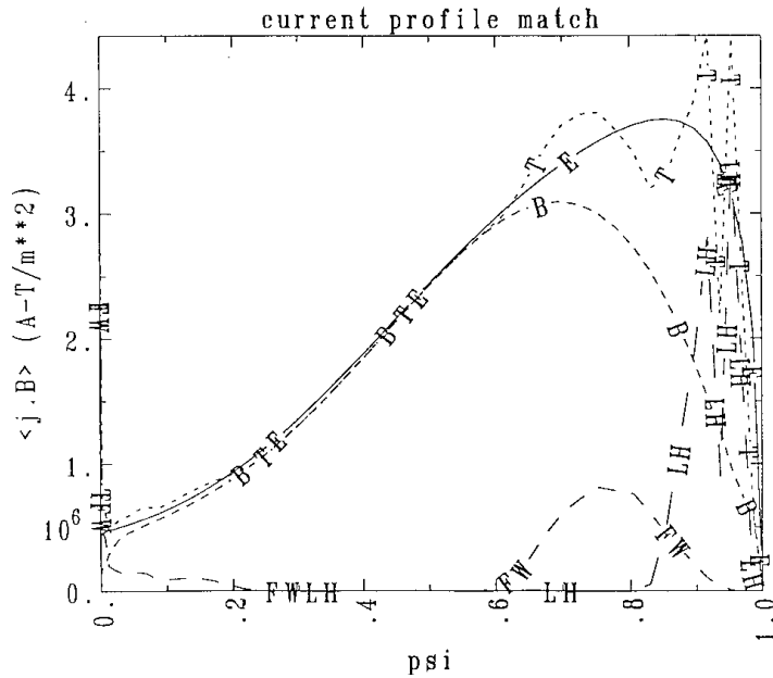
Figure 8.2-3. Current density profiles calculated from the CURRAY code for the \langle T_e \rangle = 15 keV case of Table 8.2-III. Curves labeled E, B, FW, LH and T correspond to equilibrium, bootstrap, fast-wave, lower-hybrid, and total driven current densities, respectively.
