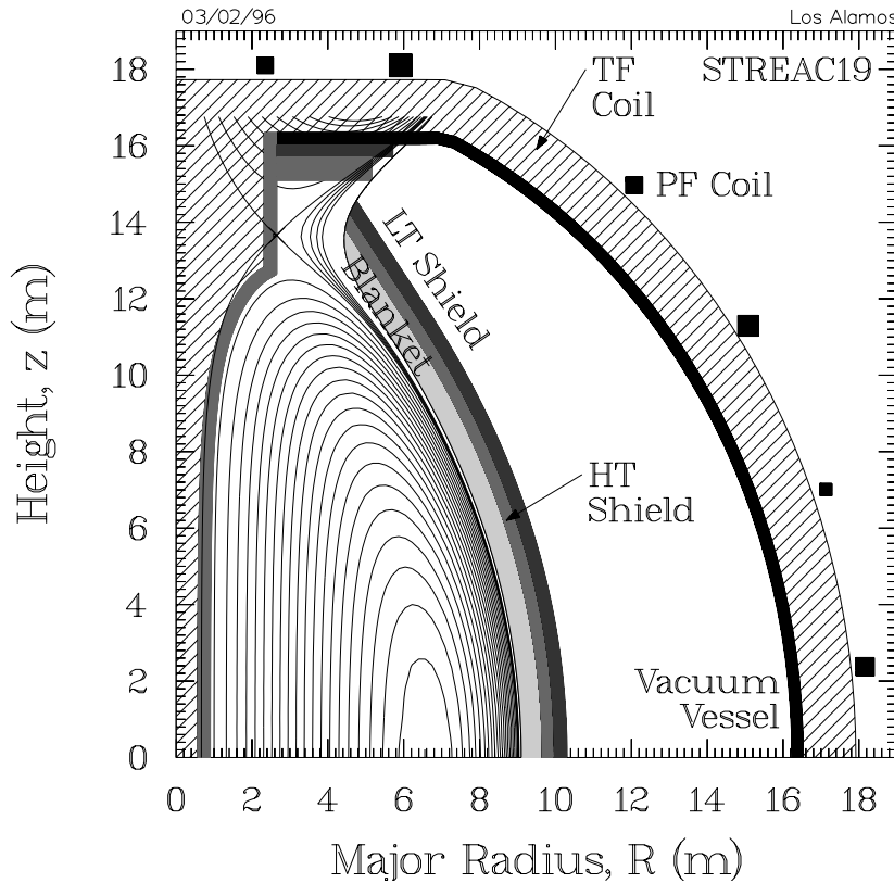
Figure 8.4-1. Elevation view of an upper-half quadrant of the LAR fusion power core.
