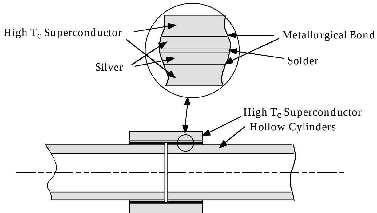
Figure 8.3-7. Schematic diagram of a joint, showing metallurgical and solder bonds.
