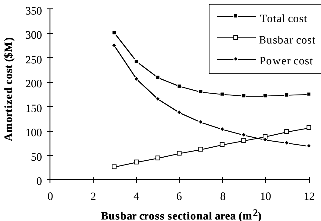
Figure 8.3-5. Amortized costs of busbar and power as a function of busbar area.
