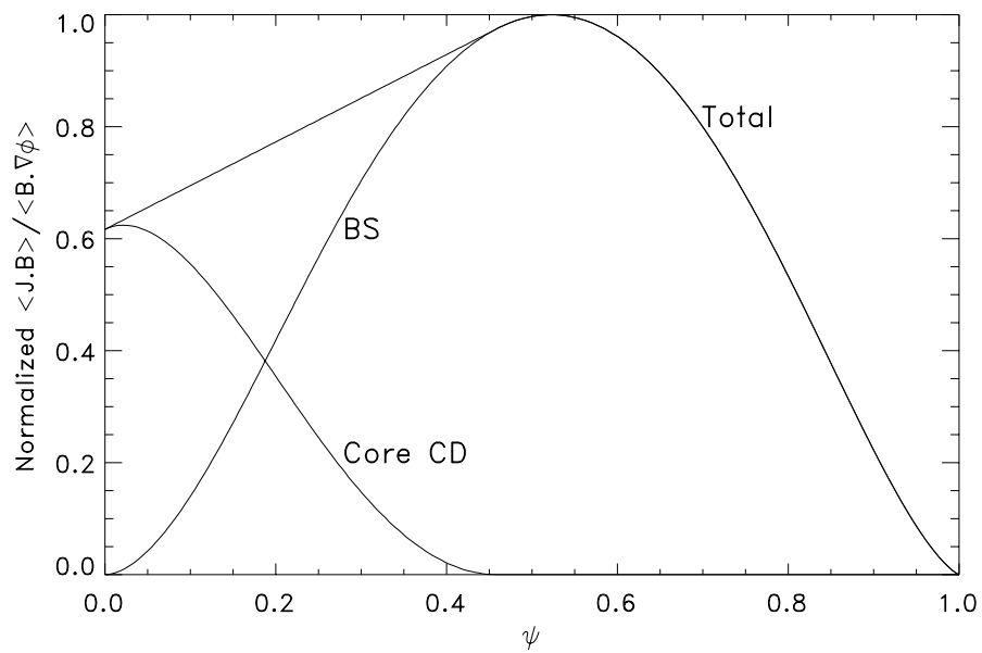
Figure 8.2-2. Parallel currents as functions of poloidal flux \psi for a high-bootstrap-fraction equilibrium which does not require edge current drive.
