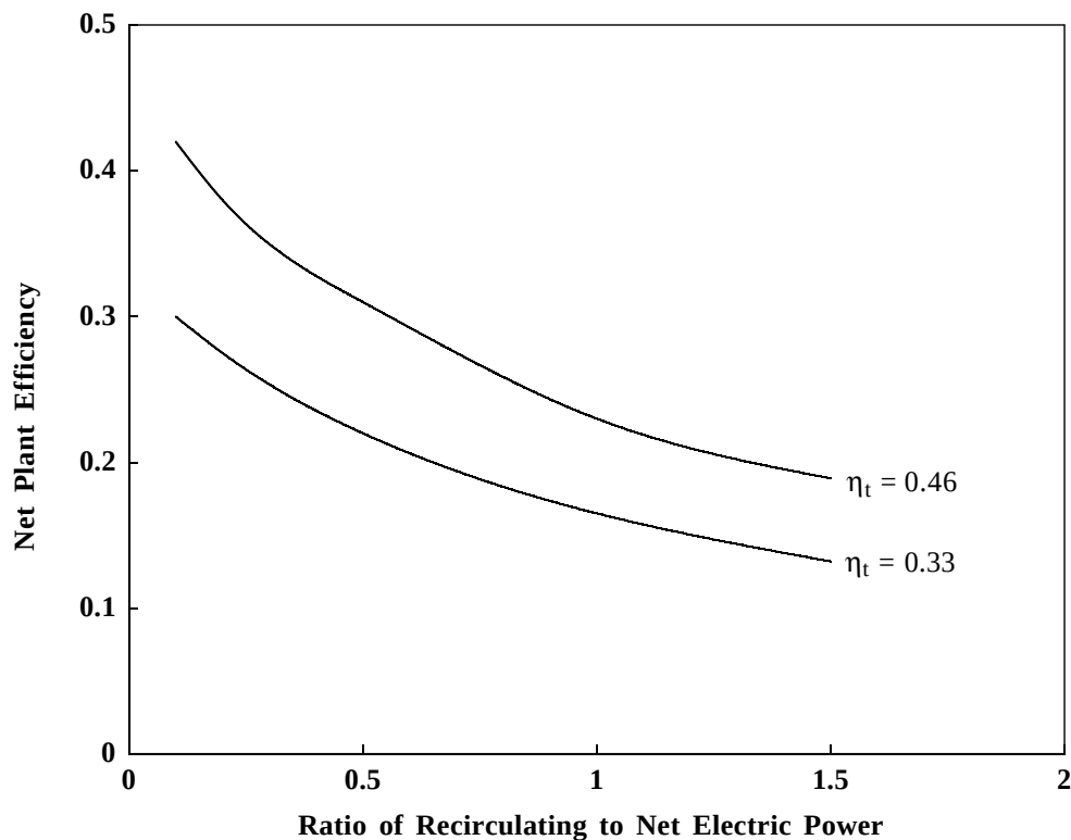
Figure 8.3-8. The net plant efficiency, \eta_{net} as a function of recirculating power fraction for different net thermal cycle efficiencies. The Starlite goal is a net plant efficiency of \sim 40\% .
