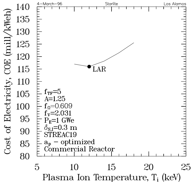
Figure 8.4-6. The cost of electricity for LAR parameters as a function of the plasma ion temperature. Each point along the curve represents the COE optimum in plasma minor radius, a_p .
