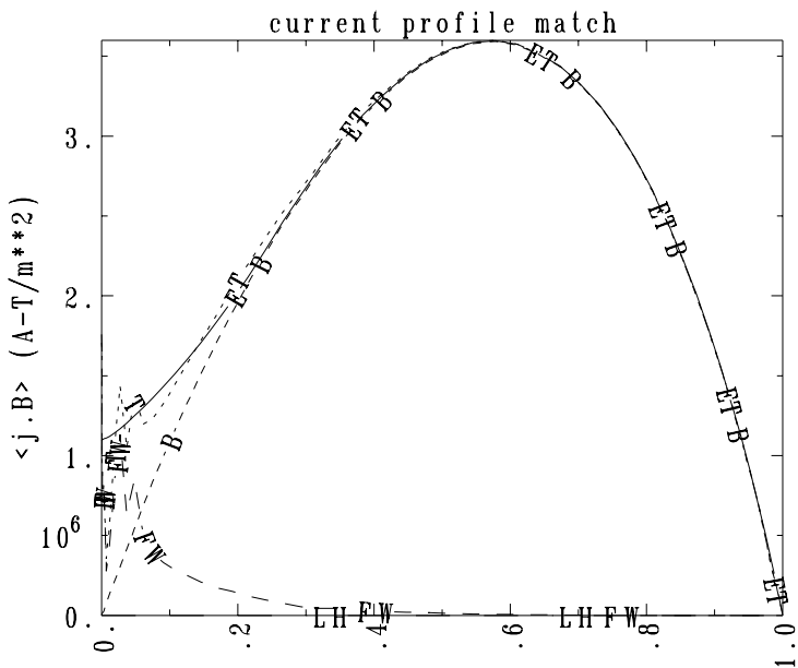
Figure 8.2-4. Current density profiles calculated from the CURRAY code for the \langle T_e \rangle = 20 keV case of Table 8.2-IV. Curves labeled E, B, FW, and T correspond to equilibrium, bootstrap, fast-wave, and total driven current densities, respectively.
