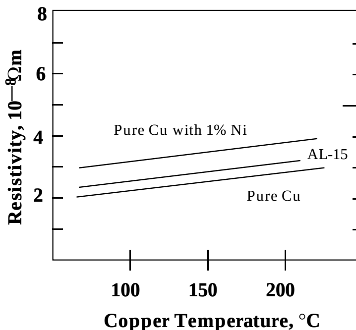
Figure 8.3-1. Resistivity of pure , dispersion-strengthened , and irradiated copper.
