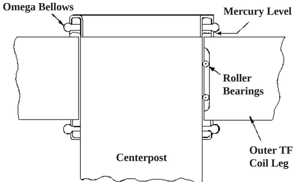
Figure 8.3-2. A possible design of a sliding electrical connection on the upper end of the center-post.
