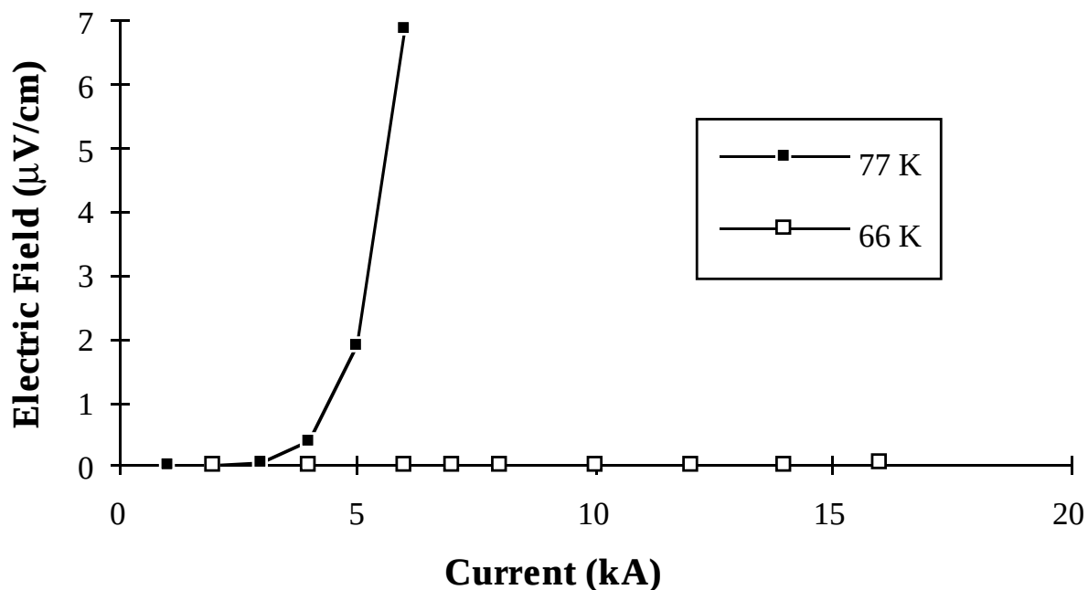
Figure 8.3-6. Electric field of high- T_c Superconductor vs current.
