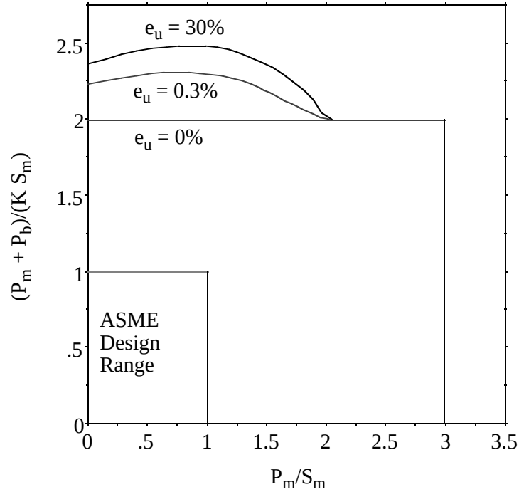
Figure 8.3-4. Safety factors for primary membrane plus bending loads as functions of primary membrane loads based on an elastic/linearly-plastic model. The assumed design properties correspond to those of unirradiated 316L(N) at 160°C: S_{ud} = 440.1 MPa, S_{yd} = 163 MPa, S_m = 147 MPa, and e_u = 30\% . A rectangular cross-section ( K = 1.5 ) is assumed. The other two cases ( e_u = 0.3\% and e_u = 0\% ) are presented to show the effects of decreasing ductility on the safety factor.
