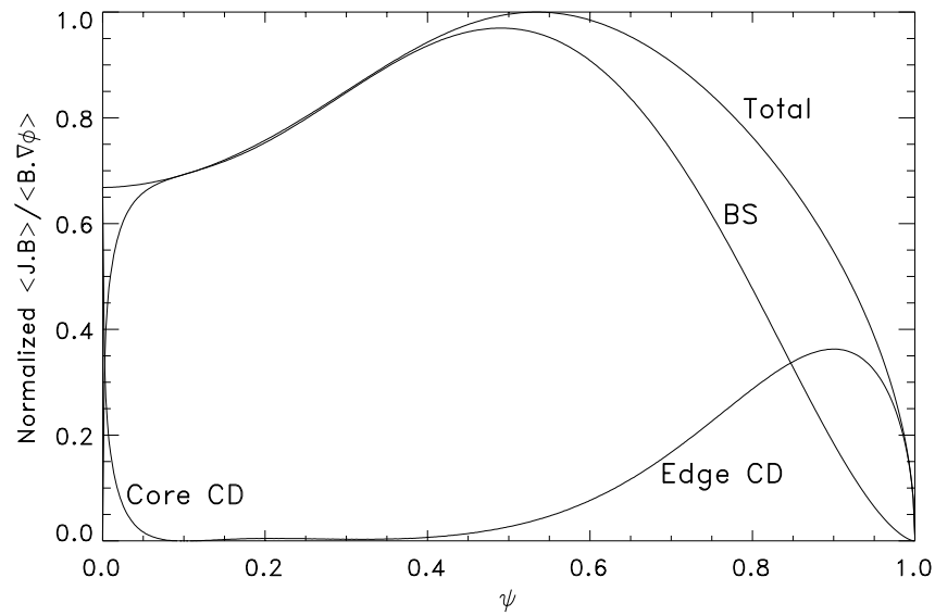
Figure 8.2-1. Parallel currents as functions of poloidal flux \psi for a high-bootstrap-fraction equilibrium which requires edge current drive.
