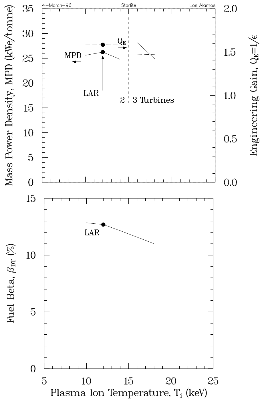
Figure 8.4-7. Variation of the mass power density (left scale, top frame) and engineering gain (right scale, top frame) and the fuel \beta (bottom frame) for the ion-temperature variation of Fig. 8.4-6.
