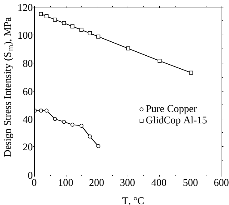
Figure 8.3-3. Design stress intensity ( S_m ) values for pure copper (C10200 in O60 temper) and GlidCop Al-15 (HIP) in the unirradiated condition.
