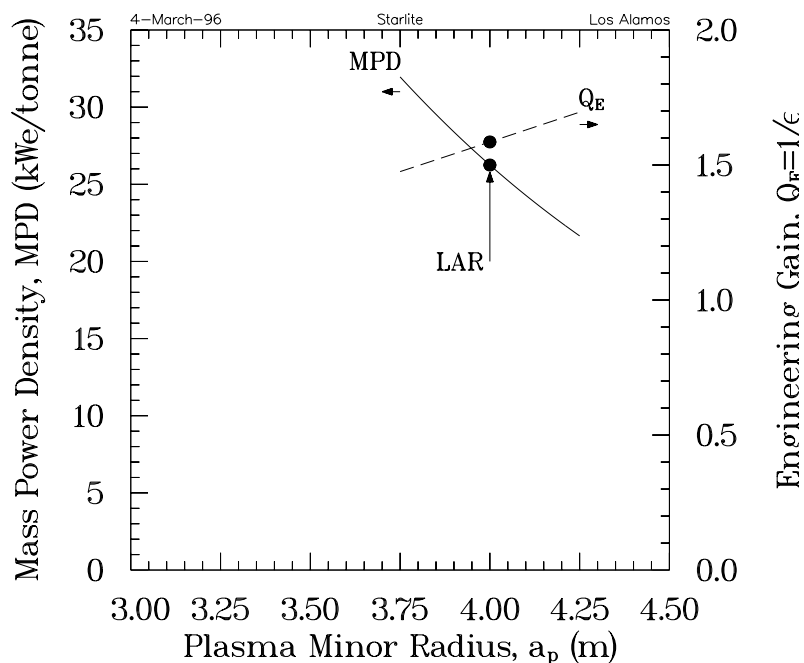
Figure 8.4-3. The mass power density (left scale) and the engineering gain (right scale) for the minor-radius variation of Fig. 8.4-2.
