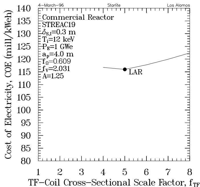
Figure 8.4-4. The cost of electricity for LAR parameters as a function of the outboard TF-coil cross-sectional scale factor.
