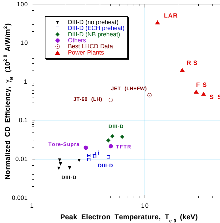
Figure 5.2-5. Fast-wave current-drive experimental database on DIII-D [21], Tore Supra [22], and TFTR [23]; best data point for lower-hybrid current-drive on JT-60 [20] and for lower-hybrid and FWCD synergy on JET [24]. Reference \gamma_B values for Starlite power plant options (FS, PU, RS, SS, and LAR) are also shown.
