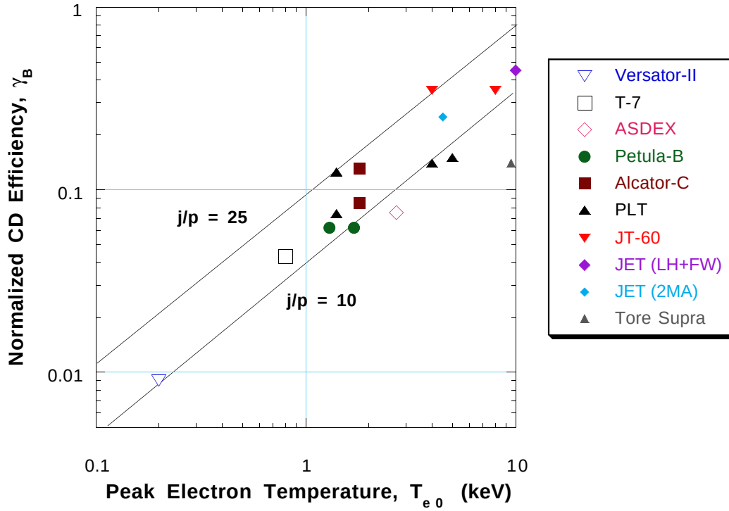
Figure 5.2-4. Experimental values of the lower-hybrid current-drive efficiency as a function of central electron temperature, T_{e0} ; for most of these experiments the bootstrap current contribution is small so \gamma_B \simeq \gamma_{CD} .
