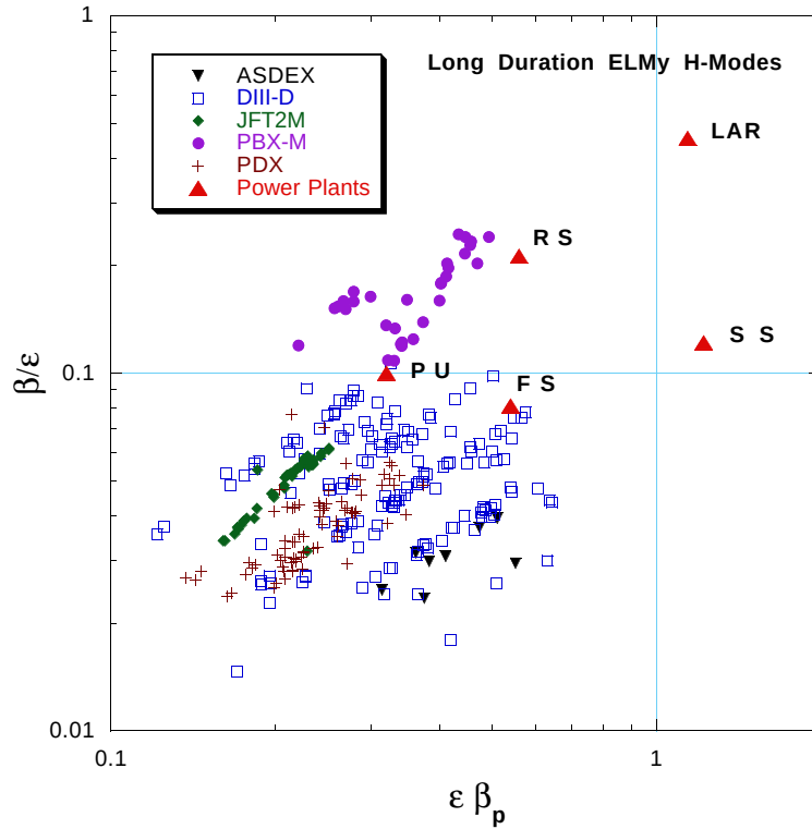
Figure 5.2-2. MHD figures of merit for long-pulse ELMy, H-mode discharges in several existing devices and the five Starlite fusion power plant options (FS, PU, RS, SS, and LAR).
