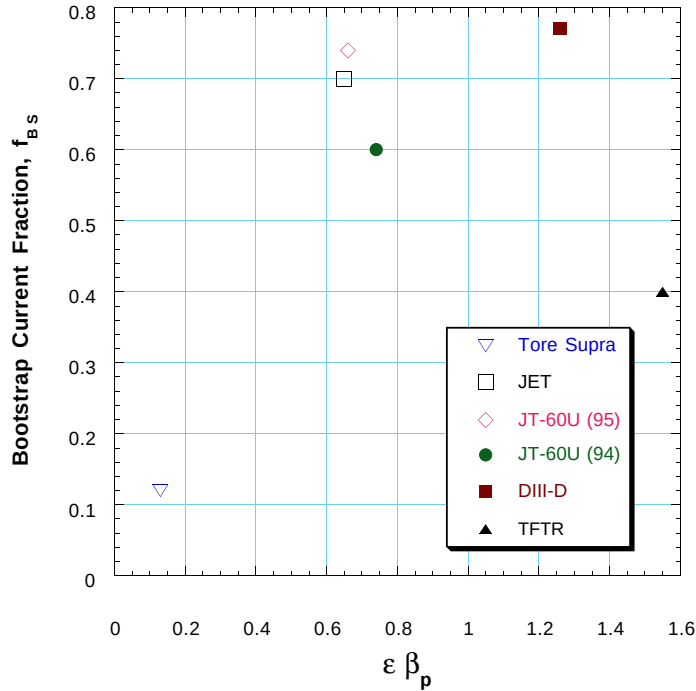
Figure 5.2-3. Large tokamak experiments which display substantial bootstrap fraction at high poloidal beta. Note that poloidal beta definitions vary somewhat; and plasma conditions (collisionality, density gradient, impurity content, etc. ) also vary.
