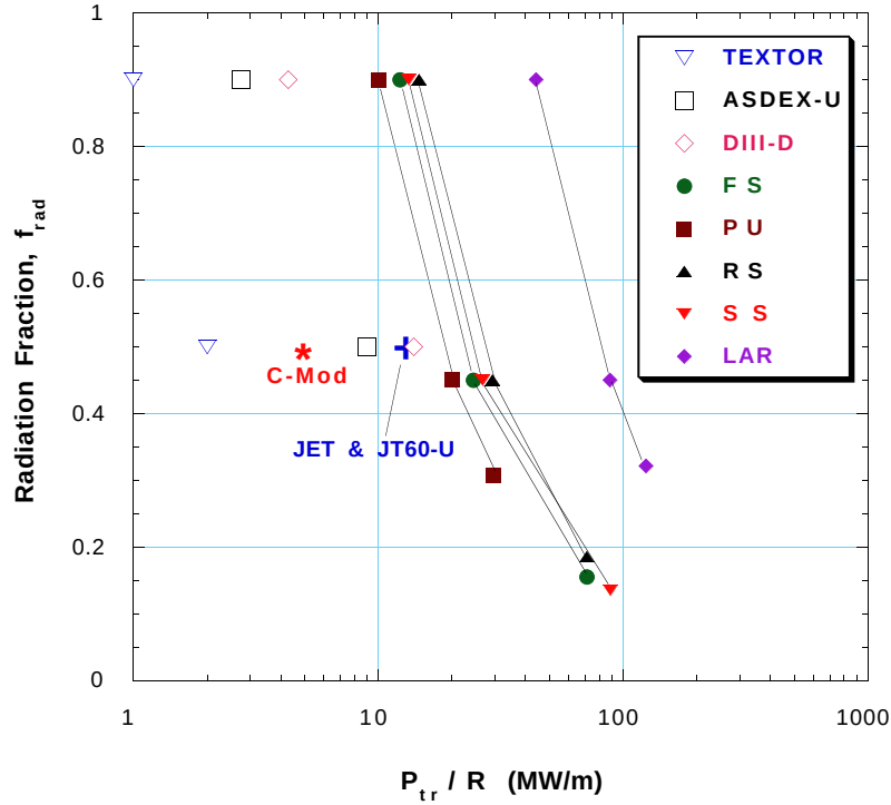
Figure 5.2-8. Plot of heat exhaust figures of merit, f_{rad} versus P_{tr}/R , for a number of present experiments (TEXTOR, C-Mod, JET, JT60-U, ASDEX-U, and DIII-D), and design values for the five Starlite fusion power plant options (FS, PU, RS, SS, and LAR). The dotted and chain-dotted lines represent the trend of PU option and LAR respectively due to the variation of f_{rad} . Options FS, RS, and SS follow the chained line. Note that f_{rad} of PU fusion power plant is relatively high compared to the other concepts because no current-drive power is required.
