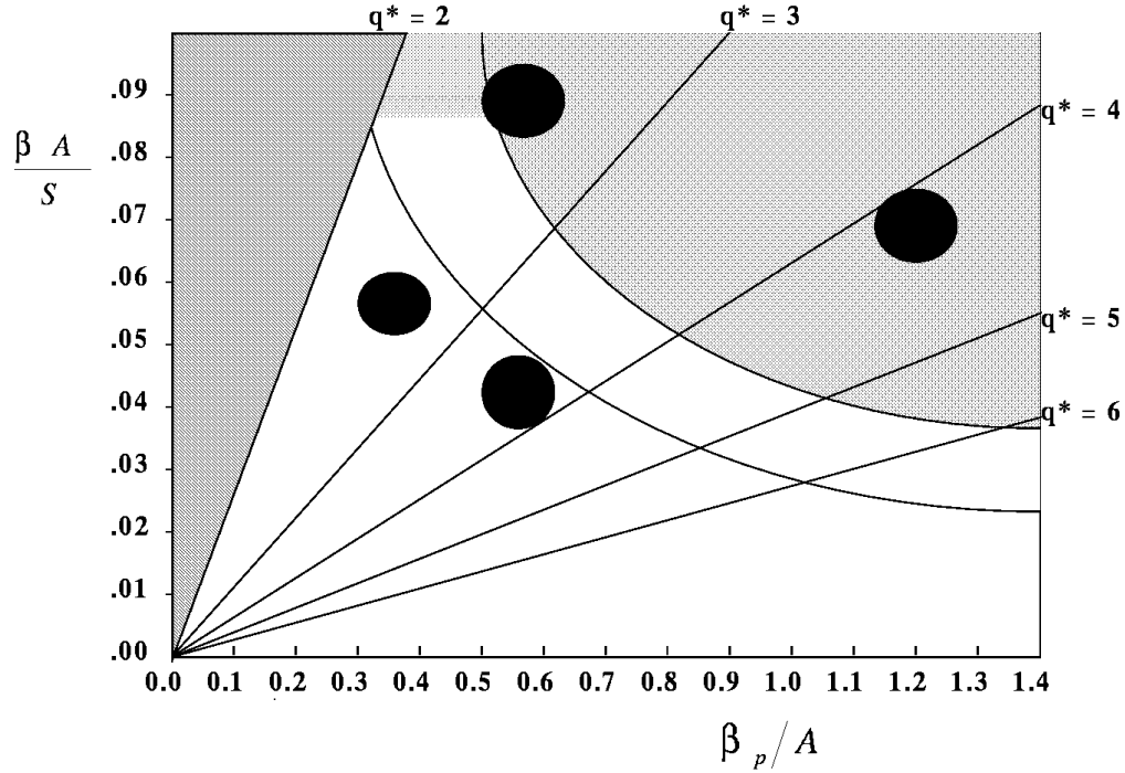
Figure 5.2-1. The MHD stability diagram showing regimes of operation for the first-stability (FS), pulsed-plasma (PU), reversed-shear (RS), and second-stability (SS) Starlite power plant options. The LAR regime is outside of this diagram, with \epsilon\beta_p \sim 1 .
