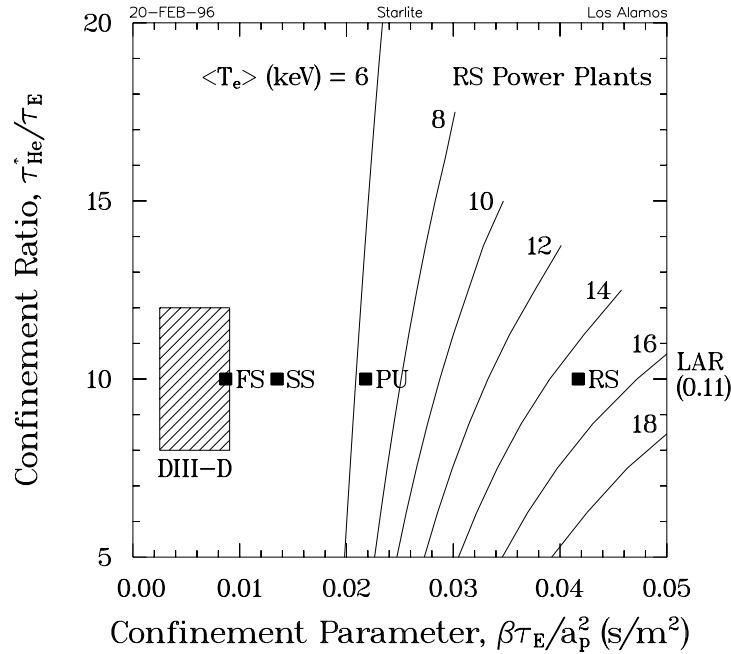
Figure 5.2-9. Ratio of effective ash confinement to energy confinement time required for power balance as the averaged plasma temperature and the ratio of ash to fuel ion densities are varied. An oxygen impurity concentration of 1% is assumed.
