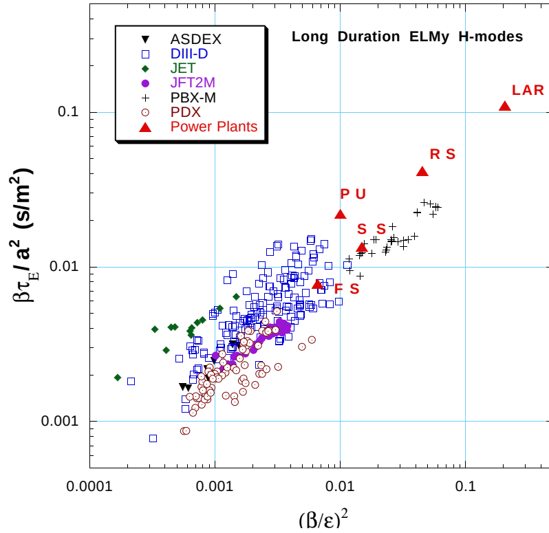
Figure 5.2-7. Energy confinement figures of merit for a number existing tokamaks and the Starlite fusion power plants. (Data provided by Stan Kaye, PPPL.)
