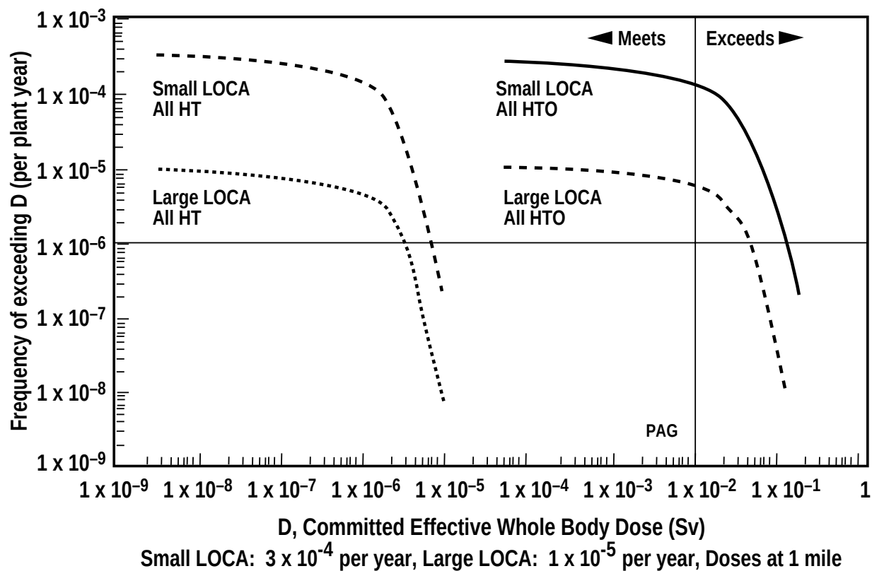
Figure 4.5-3. Preliminary ARIES-IV hazard assessment results compared to PAG (Break in the ARIES-IV helium-coolant line).
