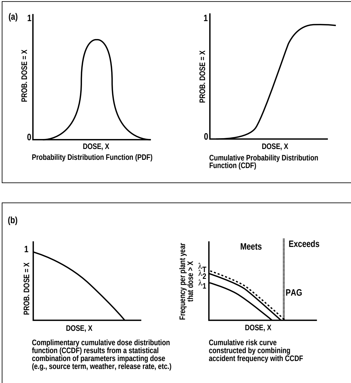
Figure 4.5-2. Description of probability distribution functions as first step in cumulative risk curve.
