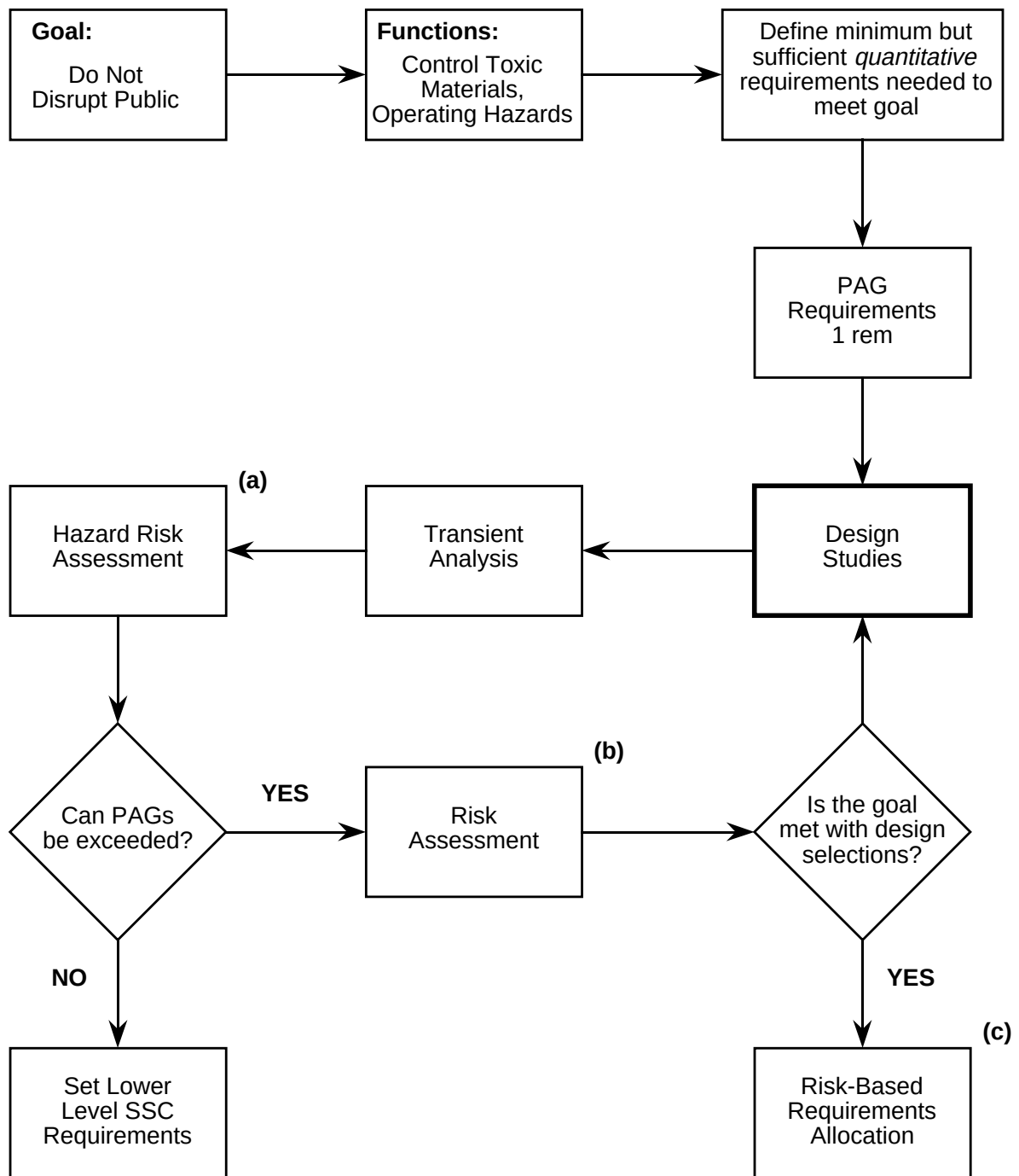
Figure 4.5-1. Logic for designing fusion facility to meet Protective Action Guidelines (PAG) requirement. The goal is to avoid “risk assessment” by meeting PAG requirements by using low-activation material and care in design.
