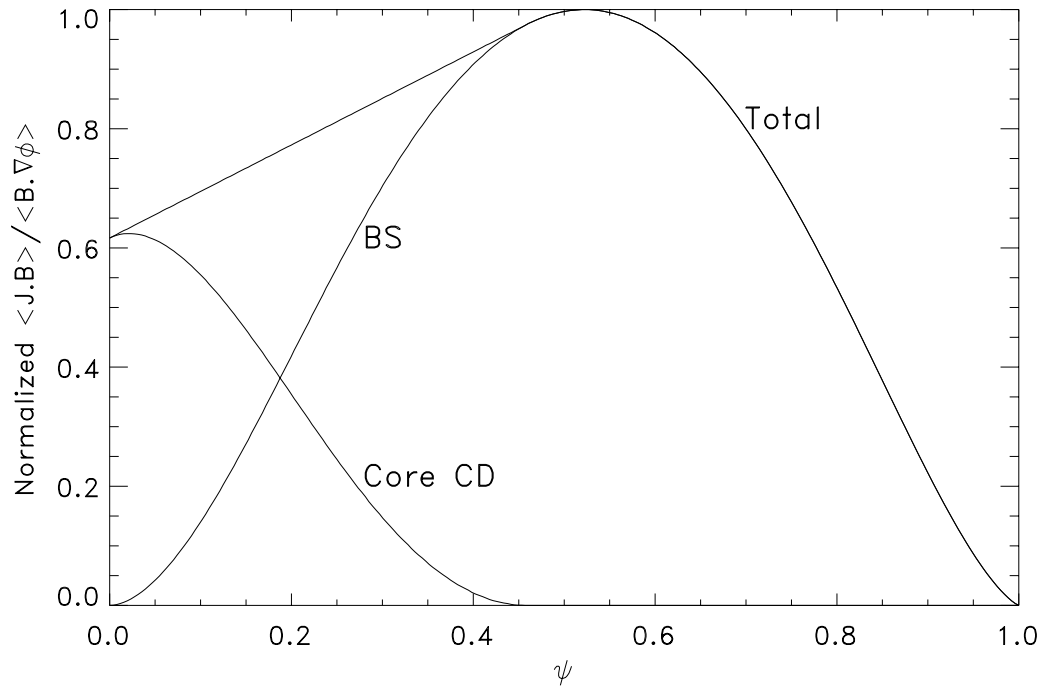
Figure 1.3-1. Parallel currents as functions of poloidal flux \psi for a high-bootstrap-fraction spherical tokamak equilibrium which does not require edge current drive.
