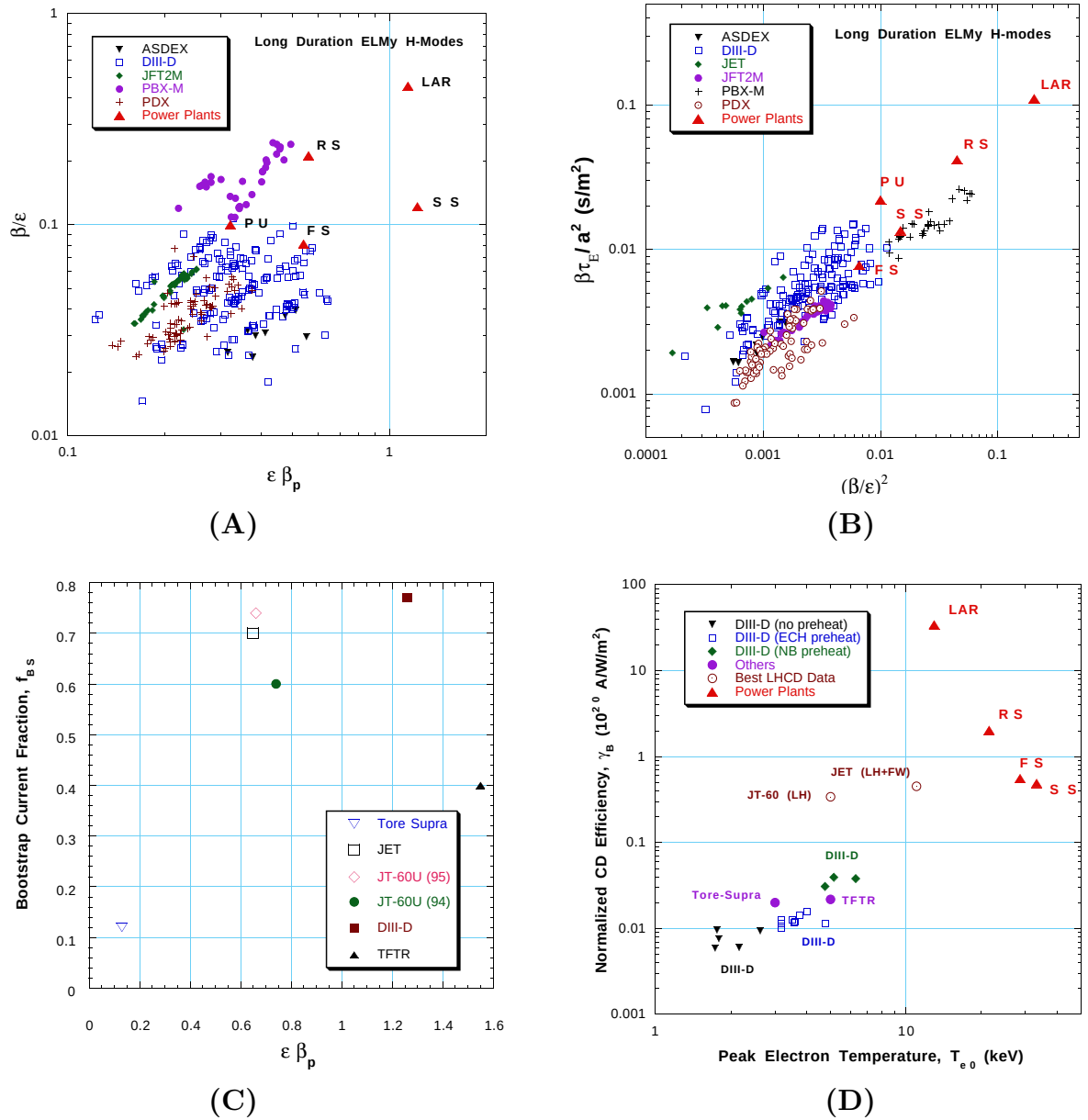
Figure 1.3-2. (A) MHD figures of merit for long-pulse ELMy, H-mode discharges in several existing devices; (B) Energy confinement figures of merit for a number existing tokamaks (Data provided by Stan Kaye, PPPL); (C) Large tokamak experiments which display substantial bootstrap fraction at high poloidal beta [Note that poloidal beta definitions vary somewhat; and plasma conditions (collisionality, density gradient, impurity content, etc. ) also vary]; (D) Fast-wave current-drive experimental database on DIII-D [14], Tore Supra [15], and TFTR [16]; best data point for lower-hybrid current-drive on JT-60 [17] and for lower-hybrid and FWCD synergy on JET [18]. The five Starlite fusion power plant options (FS, PU, RS, SS, and LAR) are also shown.
