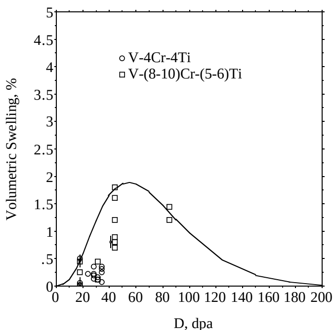
Figure A.8-1. Swelling data for V-4Cr-4Ti and V-(8-10)Cr-(5-6)Ti alloys in the temperature range of 420–600 °C and the helium concentration range of 0–75 appm. The recommended design correlation for V-4Cr-4Ti is indicated by the solid line. The curve is an upper bound to the V-4Cr-4Ti data, a reasonable bounding curve to the higher swelling V-(8-10)Cr-(5-6)Ti alloys, and follows the general shape used to describe V alloy swelling. Data for V-15Cr-5Ti (not shown) which have been used to support low swelling at high neutron damage levels include: near-zero swelling at 114 dpa and 420 °C; negligible swelling for ion irradiations up to 250 dpa and 800 °C; and negligible swelling for dual-ion irradiations up to 200 dpa, 725 °C and 1500 appm He.
