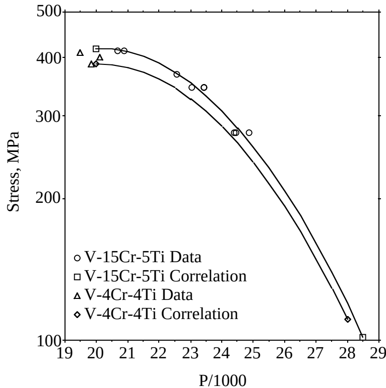
Figure A.6-1. Rupture stress as a function of the Larsen Miller Parameter, P , for V-15Cr-5Ti and V-4Cr-4Ti. The correlation for V-4Cr-4Ti is based on the form of the correlation for V-15Cr-5Ti.
