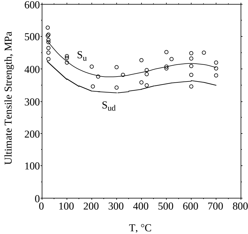
Figure A.5-1. Ultimate tensile strength (UTS) data and best-fit correlation ( S_u ) for unirradiated vanadium alloys with 4 to 5wt.% Cr, 3 to 5 wt.% Ti and 0.05 \pm 0.04 wt.% Si. The best fit correlation is recommended to represent the average UTS for V-4Cr-4Ti. The correlation S_{ud} is recommended for design analysis and for determining the limiting stress intensity ( S_m ) for average primary membrane stresses.
