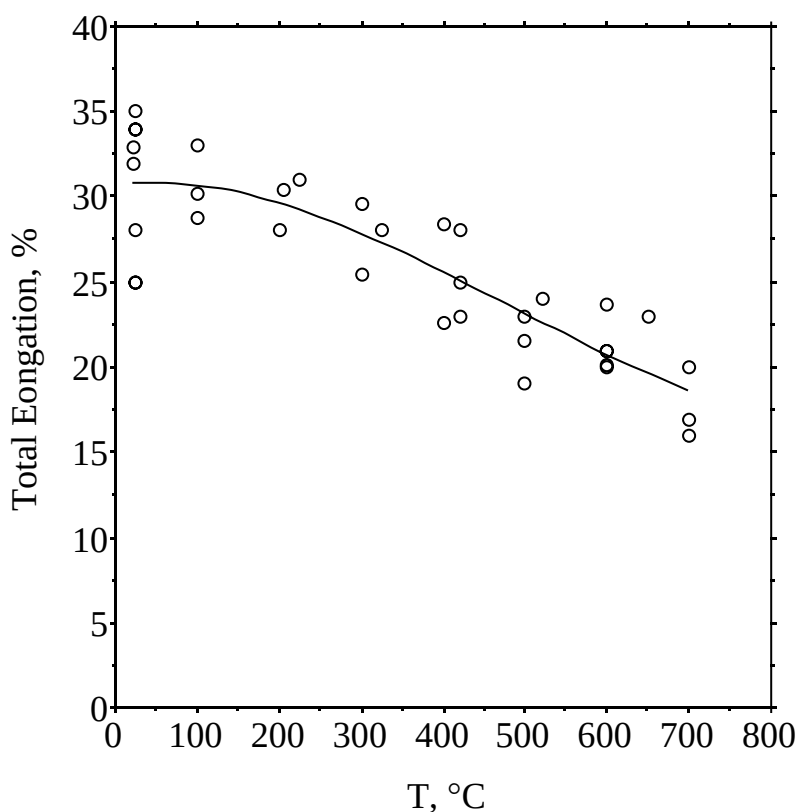
Figure A.5-4. Total elongation (TE) data and best-fit correlation for unirradiated vanadium alloys with 4–5 wt.% Cr, 3–5 wt.% Ti and 0.05 \pm 0.04 wt.% Si. The best fit correlation is recommended to represent the average TE for V-4Cr-4Ti.
