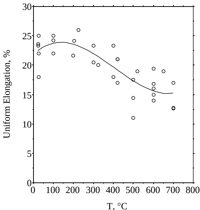
Figure A.5-3. Uniform elongation (UE) data and best-fit correlation for unirradiated vanadium alloys with 4–5 wt.% Cr, 3–5 wt.% Ti and 0.05 \pm 0.04 wt.% Si. The best fit correlation is recommended to represent the average UE for V-4Cr-4Ti.
