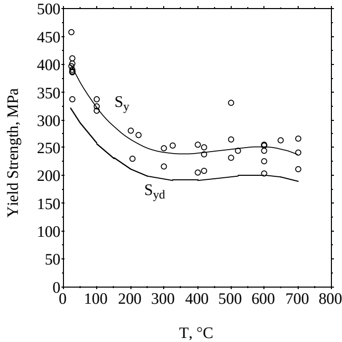
Figure A.5-2. Yield strength (YS) data and best-fit correlation ( S_y ) for unirradiated vanadium alloys with 4–5 wt.% Cr, 3–5 wt.% Ti and 0.05 \pm 0.04 wt.% Si. The best fit correlation is recommended to represent the average YS for V-4Cr-4Ti. The correlation S_{yd} is recommended for design analysis and for determining the limiting stress intensity ( S_m ) for average primary membrane stresses.
