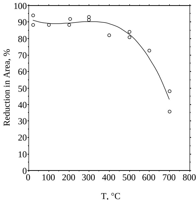
Figure A.5-5. Reduction in area (RA) data and best-fit correlation for unirradiated vanadium alloys with 4-5 wt.% Cr, 3-5 wt.% Ti and 0.05 \pm 0.04 wt.% Si. The best fit correlation is recommended to represent the average RA for V-4Cr-4Ti.
