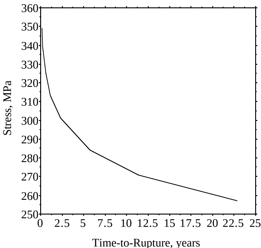
Figure A.6-2. Predicted stress as a function of rupture time for V-4Cr-4Ti at 700 °C based on the Larsen-Miller-Parameter correlation shown in Fig. A.6-1.
